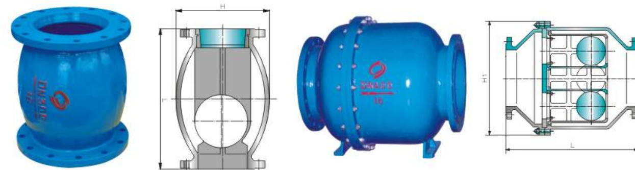
HQ44X-16 DN50-350
