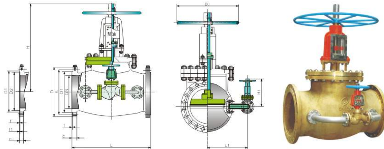
● Jyu41W-25P(T)型氧气、氮气、氩气专用截止阀 Oxygen, nitrogen, argon dedicated globe valve
